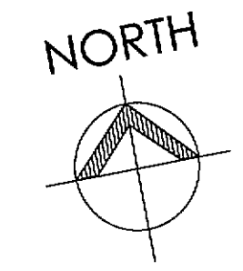
SHADOW DIAGRAM - MAR/SEP 22nd - 9AM SCALE 1: 200 @ B1
